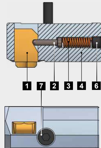
Kazeta SNAP20 >Ø 35,0 mm
